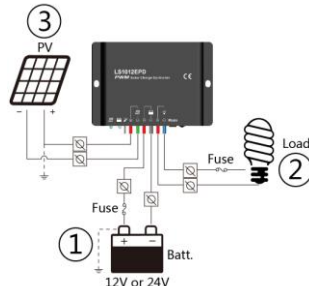
Figure1 Mounting
